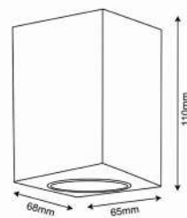
OL-SQS001-B GU10 SPOTLIGHT SURFACE FITTING
