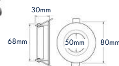
OL-821-S FIXED ROUND DOWNLIGHT FITTING ONLY WITH REMOVABLE RETAINING RING
