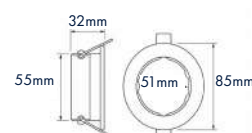
OL-8221-W & OL-8221-S FIXED ROUND DOWNLIGHT FITTING ONLY WITH RETAINING SPRING
